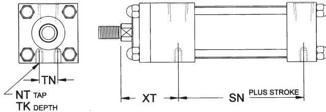
Mount Code S4 - Bottom Tapped Mount
