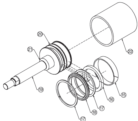
Piston/Rod Assembly
