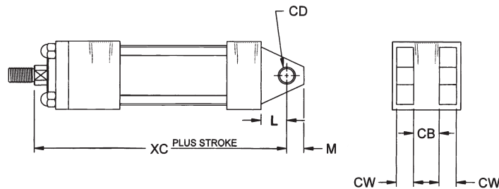
Mount Code P1 - Fixed Clevis Mount
