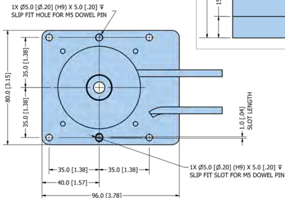
Bottom view (mPR80)
