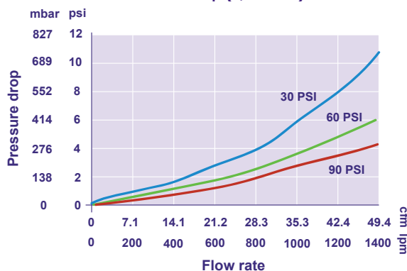
Gas flow rate Vs Pressure drop (1/2" VCR)
