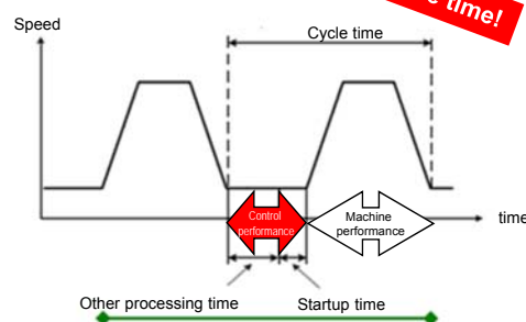
◇ Motor operation pattern example
