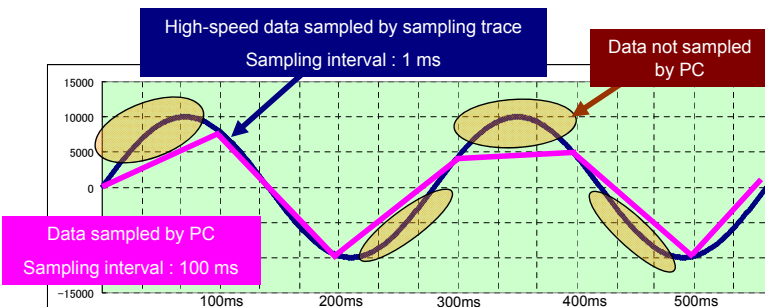
Example of data sampling using Sampling Trace: More sampled data facilitates problem analysis.
