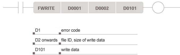
Example: FWRITE (file block write) instruction
