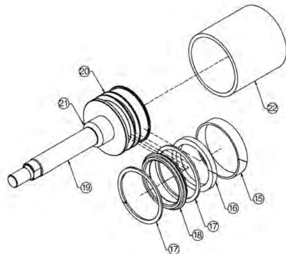
Piston/Rod Assembly
