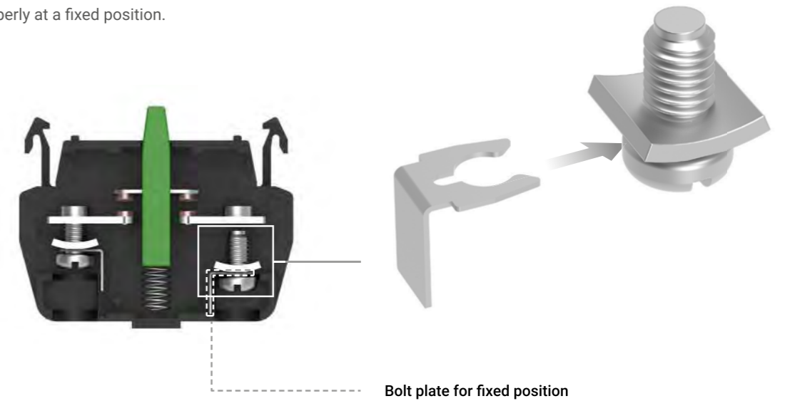
Bolt plate for fixed position
