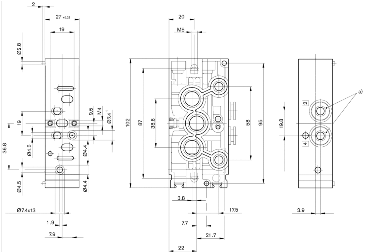
a) push-in fitting or thread connection
