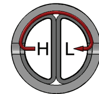
Verabar Sensor
