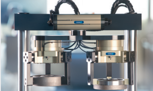
Swivel units
