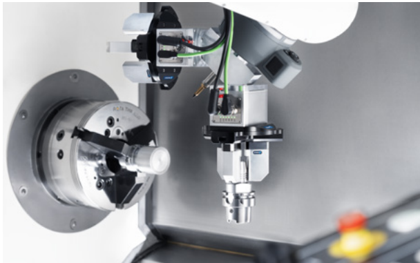
Flexible machine tool loading
