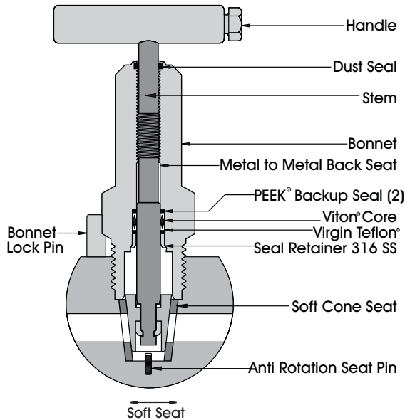
.375" Orifice
