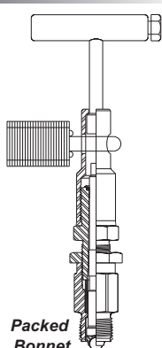
Standard Bonnet
