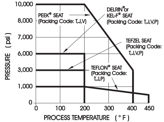
CHART D HARD SEATS - .187" and .375" ORIFICE TEFLON® PRESSURE-CORE™ SEAL and VITON O-RING SEAL All Materials
