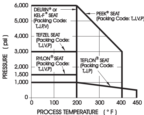
CHART E SOFT SEATS - .375" ORIFICE
