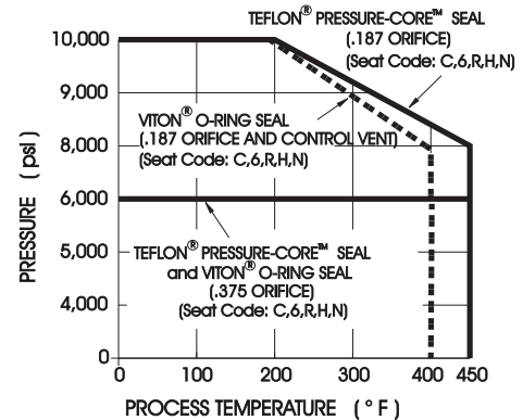
CHART D HARD SEATS - .187" and .375" ORIFICE TEFLON® PRESSURE-CORE™ SEAL and VITON O-RING SEAL All Materials
