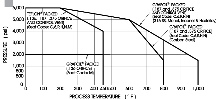
CHART F GRAFOIL® AND TEFLON® PACKED HARD SEATS - ALL ORIFICE SIZES
