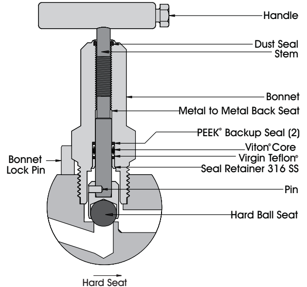
.375" Orifice
