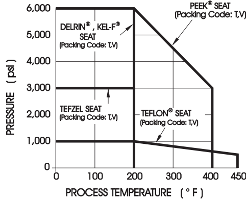
CHART C "MINI" SOFT and INTEGRAL METAL SEATS - .136" ORIFICE "T" CODE = TEFLON® PACKED and "V" CODE = VITON O-RING SEAL
